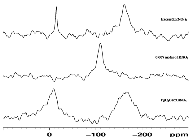
Figure 7. ^{133}\text{Cs} NMR spectra of [(\text{PgC}_4)_6\text{Ga}_{12}\text{CcsNO}_3] upon initial addition of excess potassium nitrate and subsequent addition of excess zinc nitrate.
