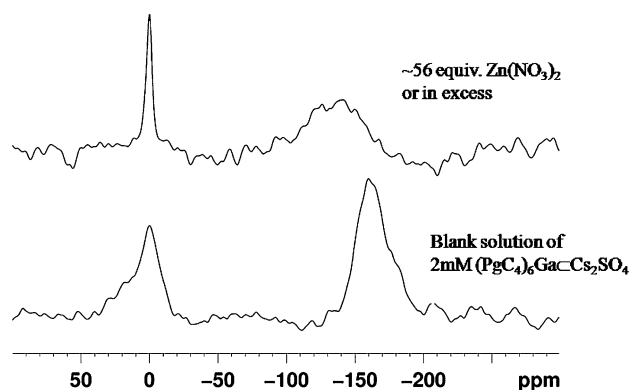
Figure 5. ^{133}\text{Cs} NMR spectra of [(\text{PgC}_4)_6\text{Ga}_{12}\text{C}\text{Cs}_2\text{SO}_4] upon titration with ethanolic zinc(II) nitrate.
